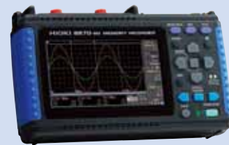
MEMORY HiCORDER 8870-20 Dual-channel (isolated) high-speed oscilloscope Measures (at 1 MS/s) and displays instantaneous AC waveforms up to 280 V External dimensions are the same as Model LR8431-20
